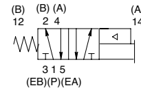
SPA single solenoid air pilot 2 position 4-way
