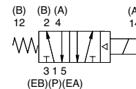
SPA single solenoid air pilot 2 position 4-way
