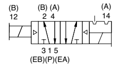
SPA double solenoid air pilot 2 position 4-way
